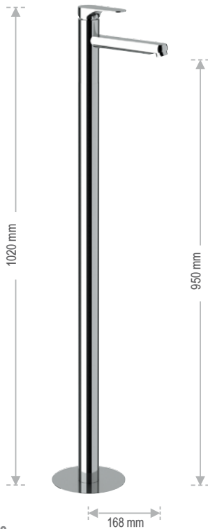
L 18 Miscelatore monocomando lavabo da terra. Single-lever mixer for floor mounting.
