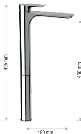
I 10 LXXL Miscelatore monocomando lavabo alto LXXL. XXL high basin mixer.
